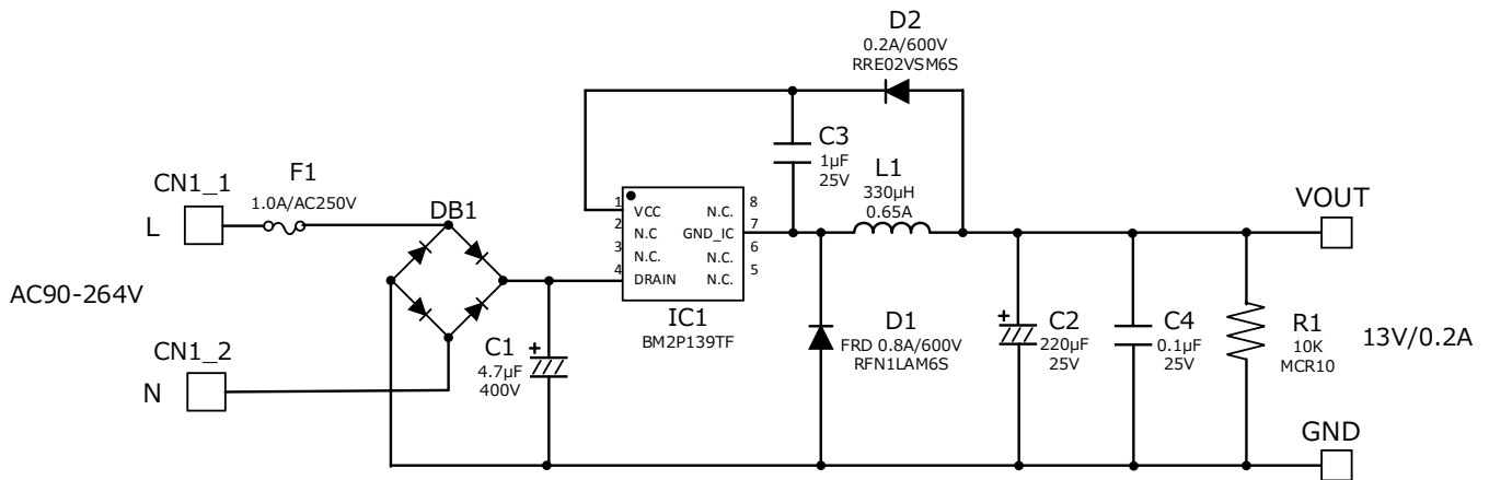
Figure 3. BM2P139TF-EVK-001 Schematics
