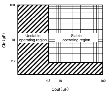
C in vs C out 1.0V \leq V O < 3.0V (Reference data)
