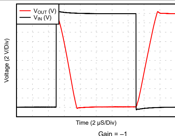
Figure 5-42. Large-Signal Step Response
