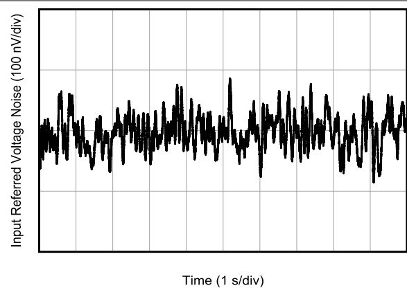
Figure 5-24. 0.1-Hz to 10-Hz Noise
