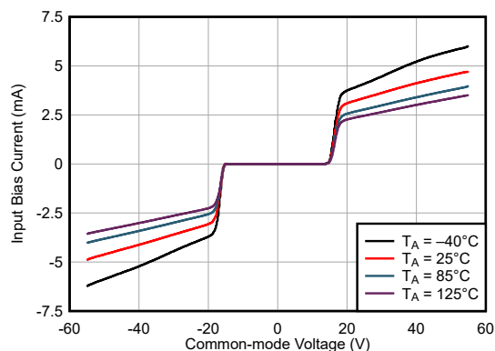
OPAx206 Input Overvoltage Protection
