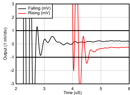
Figure 5-38. Settling Time
