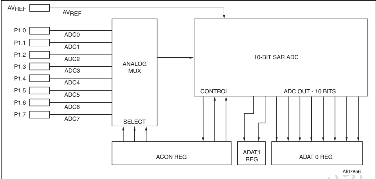
Figure 45. 10-Bit ADC
