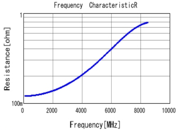
■ GJM1555C1H3R9WB01 R DC0V, 25degC
