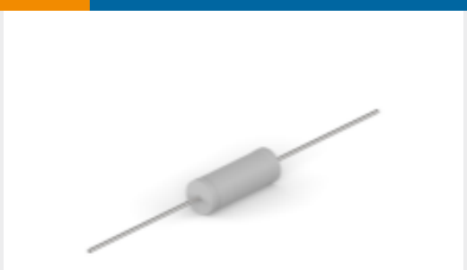
TE Part #4-2176412-6 5W XSM M/OX 5% 390R
