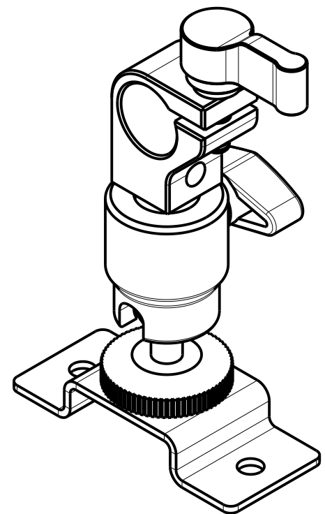
ISOMETRIC VIEW SCALE 1:1
