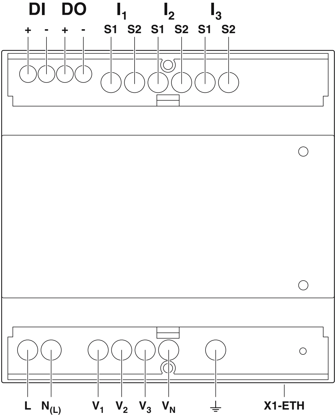
Connection diagram
