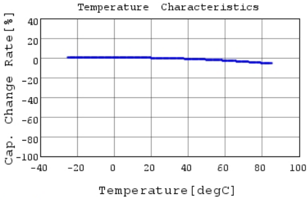
GRM155B31E473KA87 C-Temp. capchange, DC0.0V,
