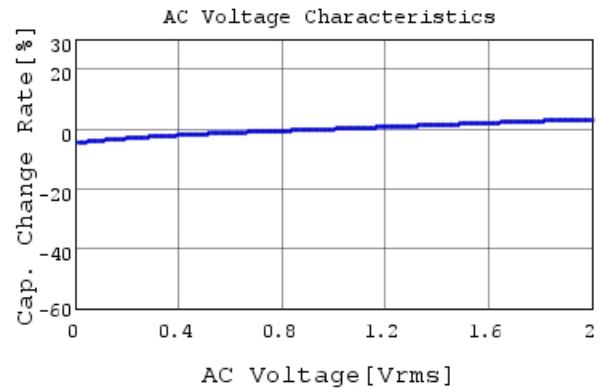
GRM155B31E473KA87 C-AC Voltage capchange, Dc
