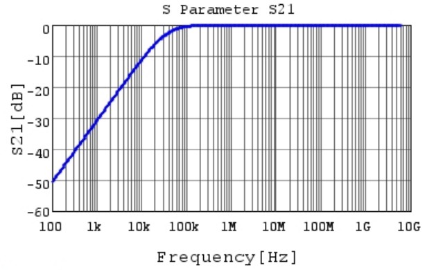
GRM155B31E473KA87 S21 DC0V, 20degC
