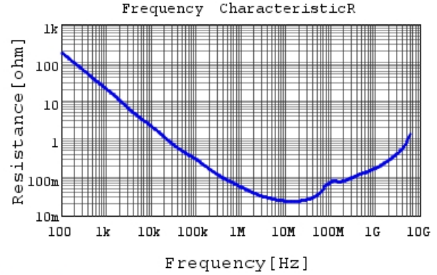
GRM155B31E473KA87 R DCOV, 20degC
