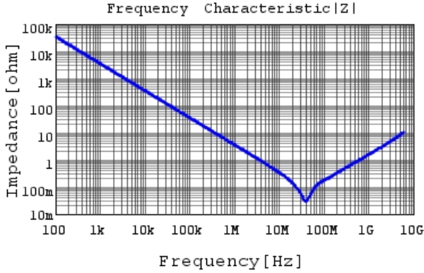
GRM155B31E473KA87 |Z| DCOV, 20degC
