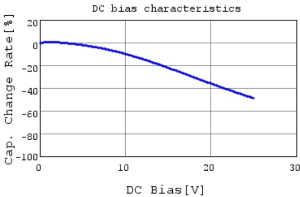
GRM155B31E473KA87 C-DC bias capchange, 20.0c
