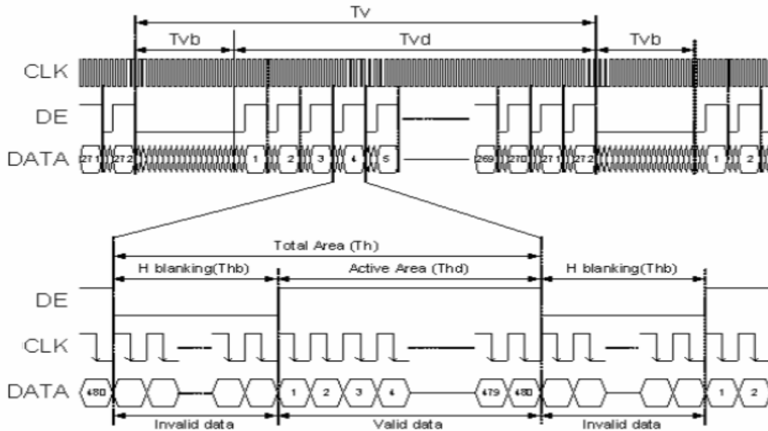
Parallel DE mode RGB input timing table
