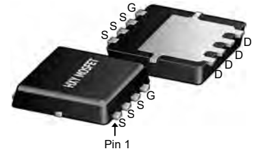
DFN5X6-8L (TDSO-8(5.9x5.2))
