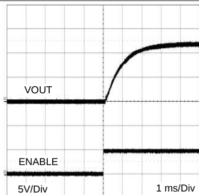
Figure 43. Startup V_{IN} = 24\text{ V} , I_{OUT} = 3\text{ A}
