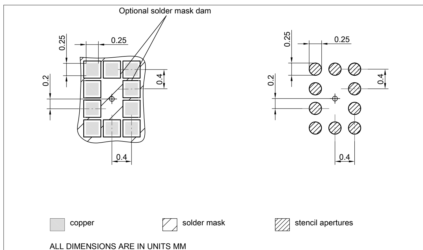
Figure 5: Footprint Recommendation
