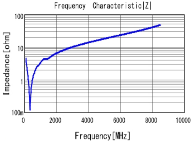
■ GRM1882C1H331JA01 |Z| DC0V, 20degC
