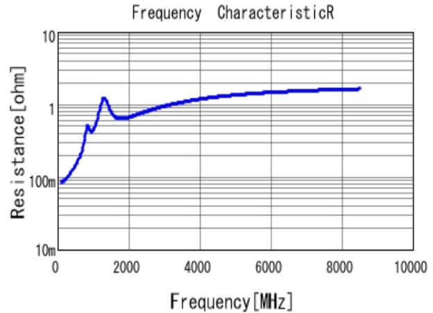
■ GRM1882C1H331JA01 R DC0V, 20degC
