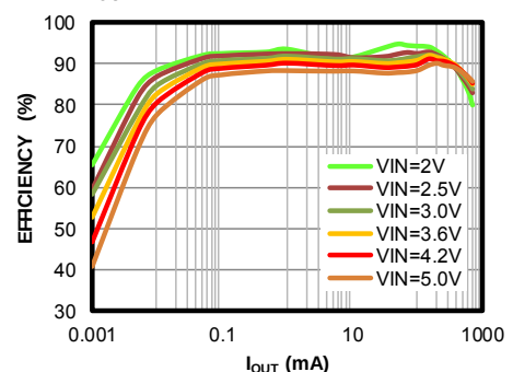
Efficiency vs. Load Current V_{OUT}=1.8V
