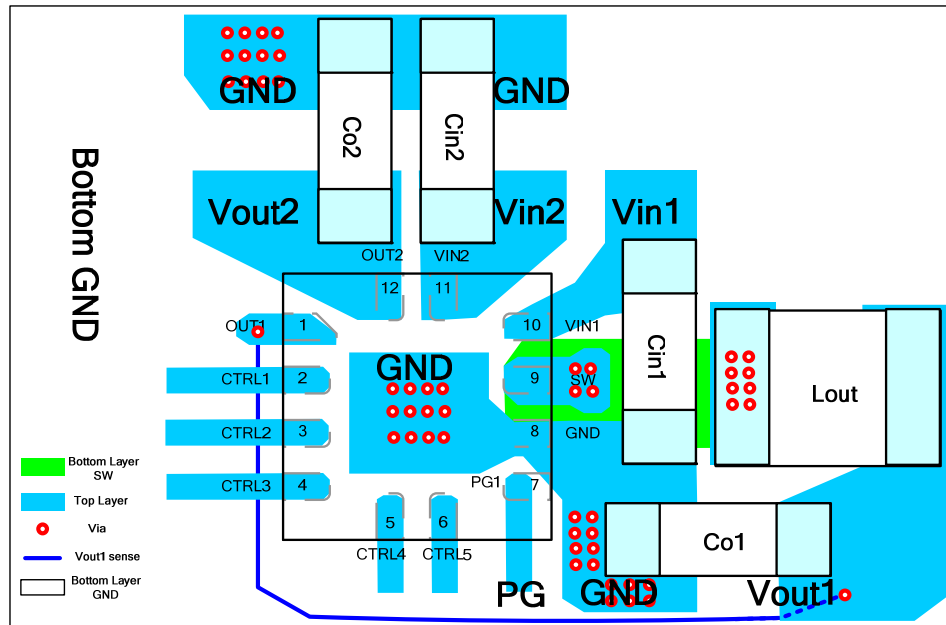
Figure 2: Recommended Layout
