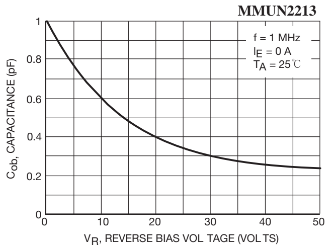
Figure 14. Output Capacitance
