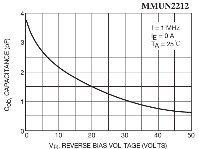
Figure 4. Output Capacitance
