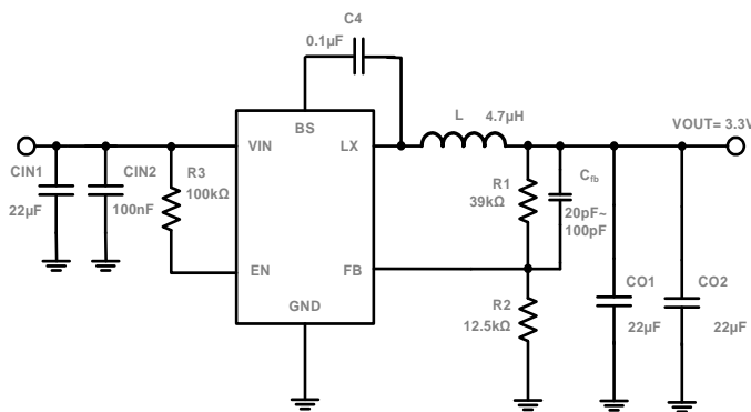
Typical Application Circuits ( V_{REF}=0.8V )
