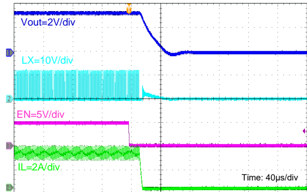
EN Disable V_{IN} = 12V , V_{OUT} = 3.3V , I_o = \text{Full Load}
