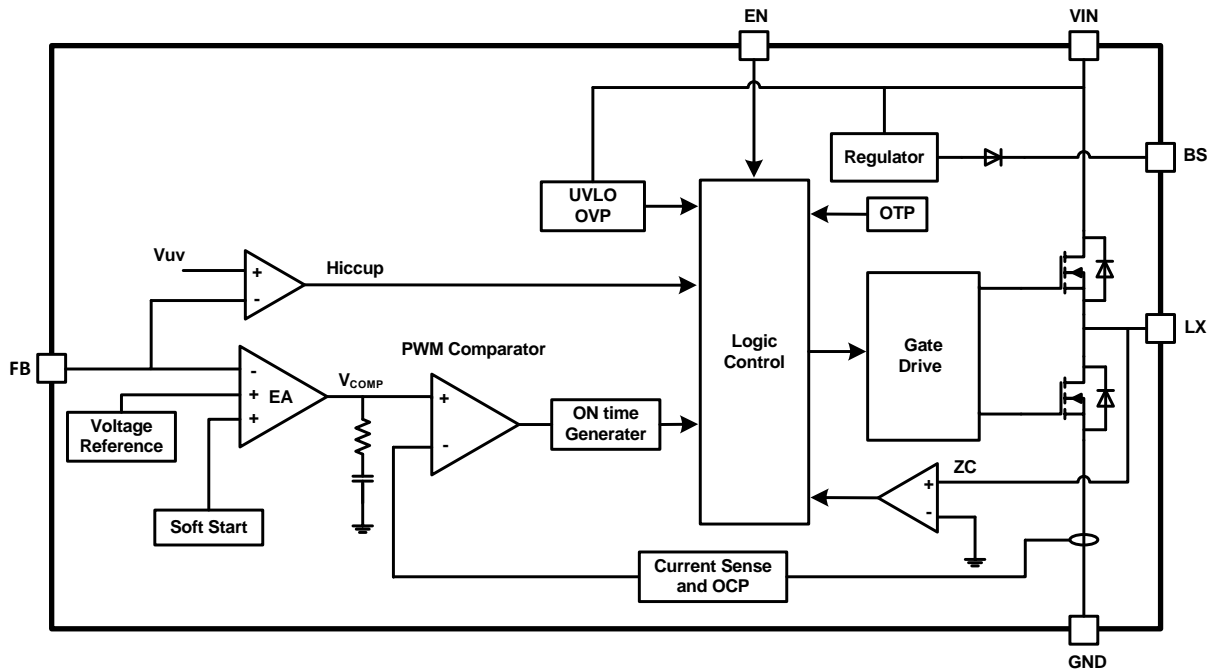
Figure 1. MP1471GJ-Z Block Diagram
