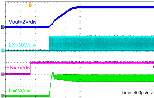
EN Enable V_{IN} = 12V , V_{OUT} = 3.3V , I_o = \text{Full Load}
