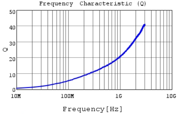
LQP02TQ2N5B02 Q
