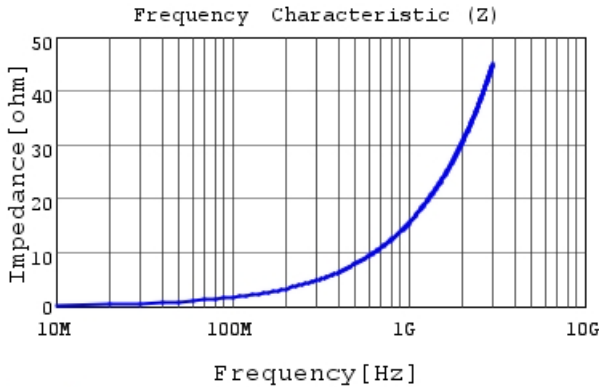
LQP02TQ2N5B02 |Z|
