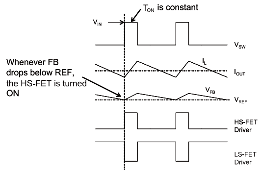
Figure 2: Heavy-Load Operation
