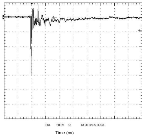
Fig.4 IEC61000-4-2 -8kV Contact Discharge
