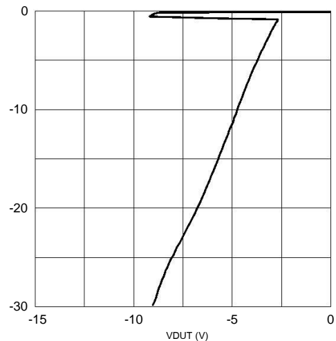
Fig.6 Transmission Line Pulse (tp=100ns)
