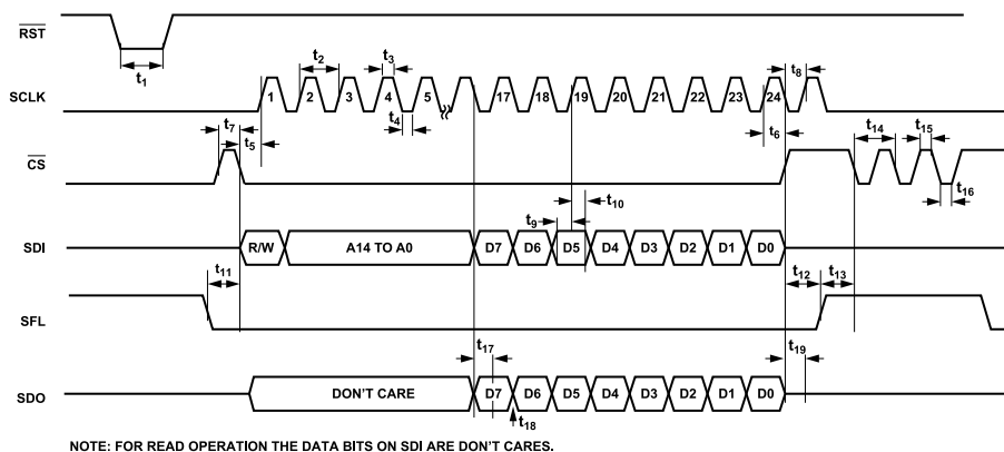
Figure 2. Timing Diagram
