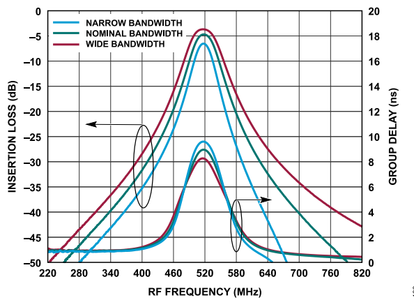
Figure 6. Insertion Loss and Group Delay vs. RF Frequency at 520 MHz
