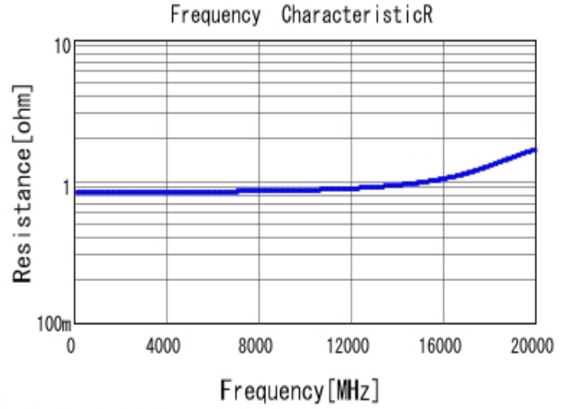
■ GRM0335C1HR70WA01 R DC0V, 25degC
