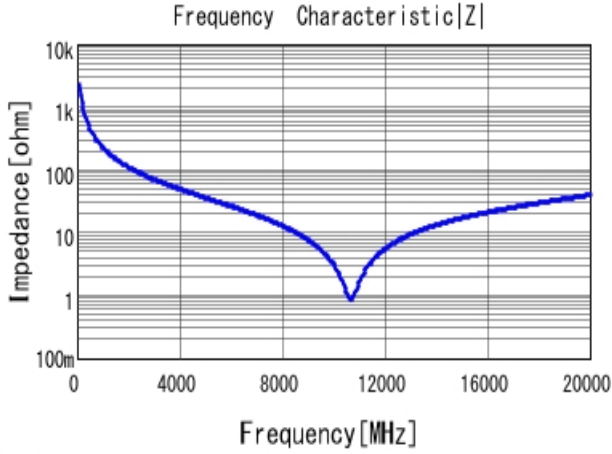
■ GRM0335C1HR70WA01 |Z| DC0V, 25degC
