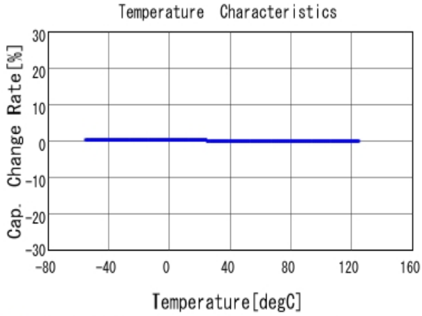
■ GRM0335C1HR70WA01 C-Temp. capchange, DCOV, AC1Vrms
