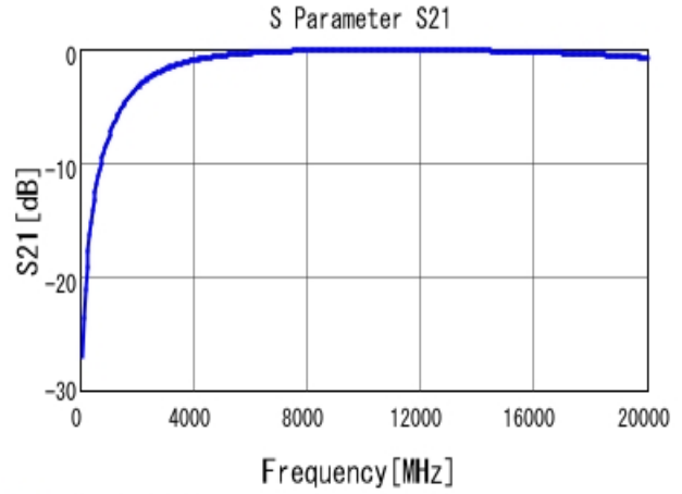
■ GRM0335C1HR70WA01 S21 DCOV, 25degC
