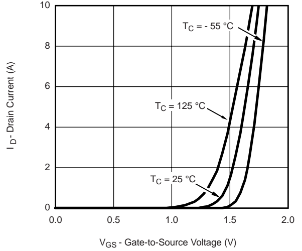
T_C = 25\text{ }^\circ\text{C} T_C = 125\text{ }^\circ\text{C} T_C = -55\text{ }^\circ\text{C} Transfer Characteristics
