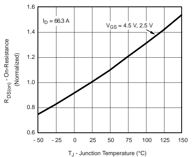
I_D = 66.3\text{ A} V_{GS} = 4.5\text{ V} V_{GS} = 2.5\text{ V} On-Resistance vs. Junction Temperature
