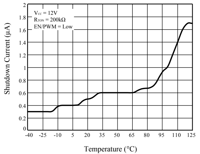
Figure 5 I_{SD} vs. Temperature
