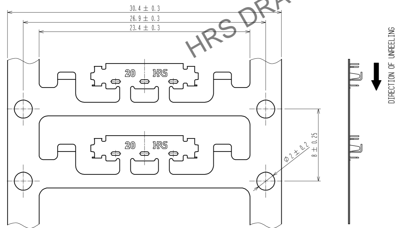
CARRIER STATE DRAWING(4:1)
