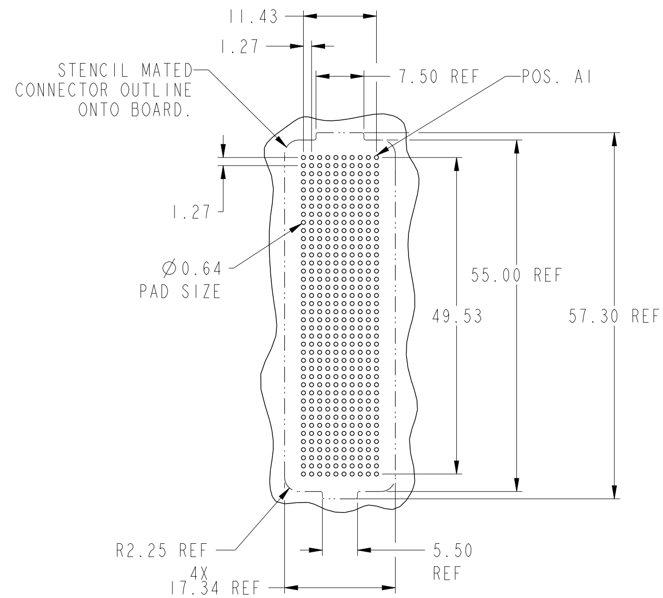
BOARD PATTERN
