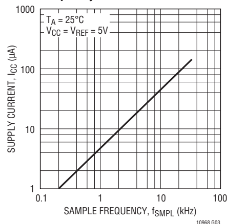
Supply Current vs Sample Frequency LTC1096
