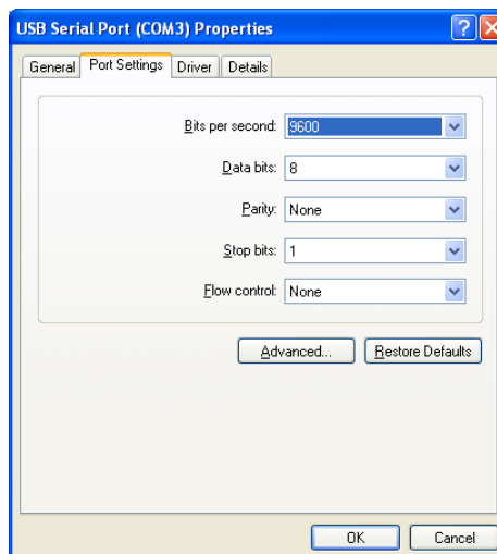
Figure 2.9 - Settings Tab
