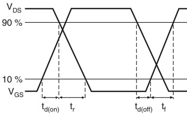
Fig. 10b - Switching Time Waveform
