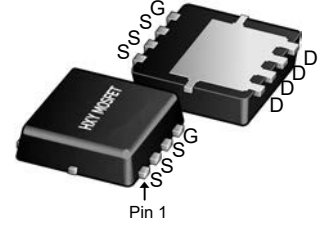
DFN3X3-8L (PowerPAK1212-8)
