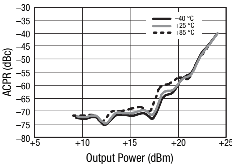
Figure 32. ACPR vs Output Power Over Temperature
