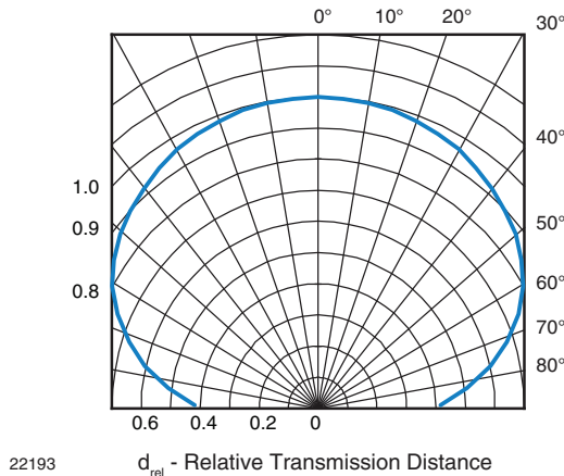
Fig. 11 - Horizontal Directivity
