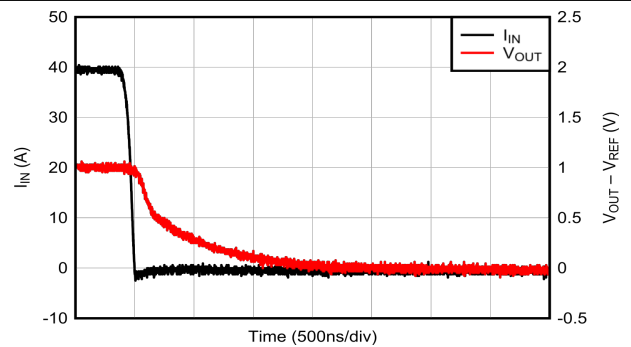
Figure 6-18. Voltage Output Step Response, Falling
