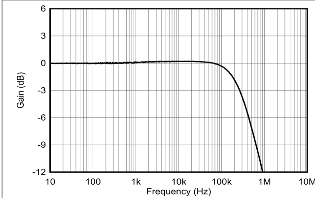
Figure 6-13. Sensitivity vs Frequency, All Gains Normalized to 1Hz
