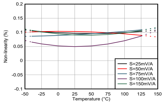
Figure 6-4. Non-Linearity vs Temperature
