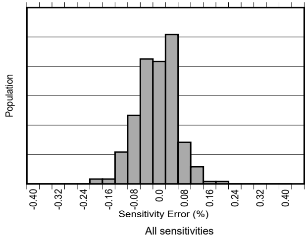
Figure 6-5. Sensitivity Error Production Distribution
