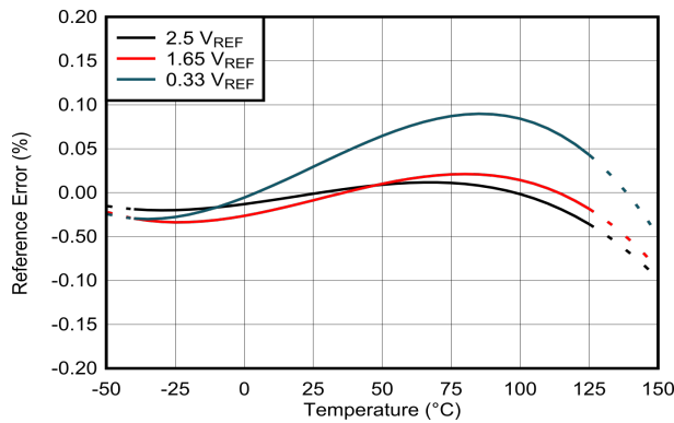
Figure 6-3. Reference Error vs Temperature
