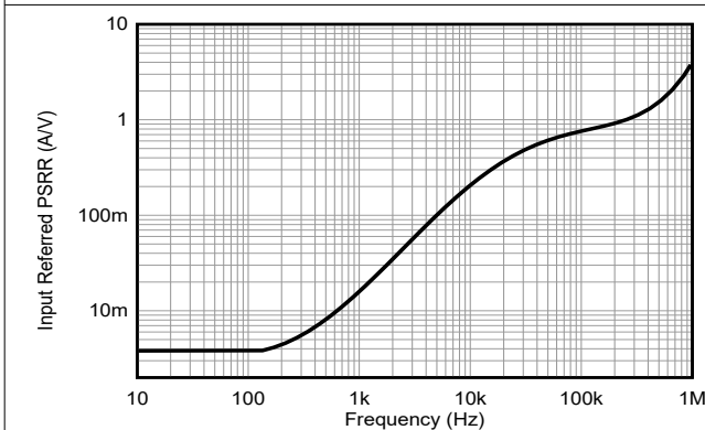
Figure 6-15. PSRR vs Frequency
