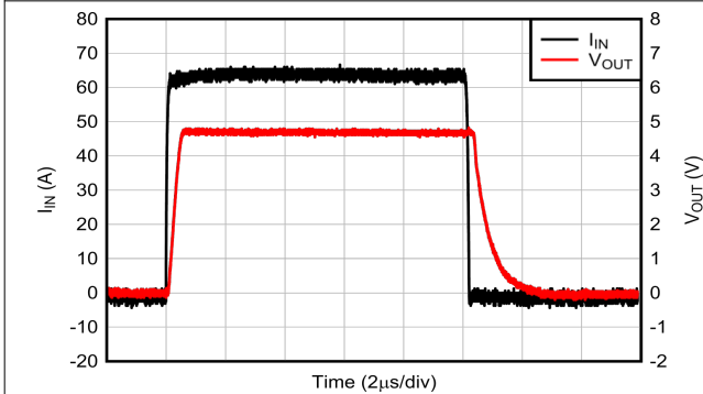
Figure 6-19. Current Overload Response
