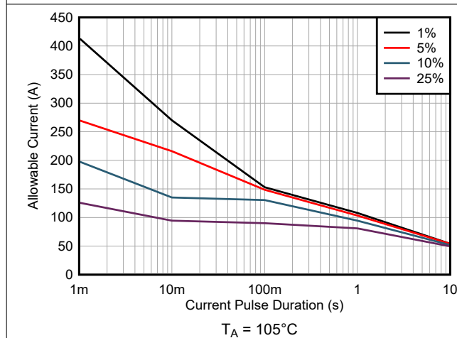
Figure 7-7. Maximum Repetitive Pulsed Current vs. Pulse Duration
