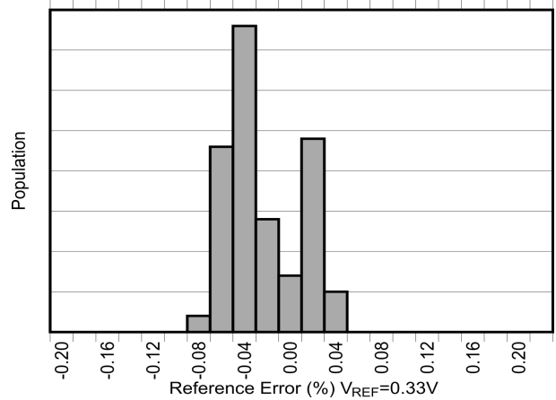
Figure 6-12. Reference Error Production Distribution
