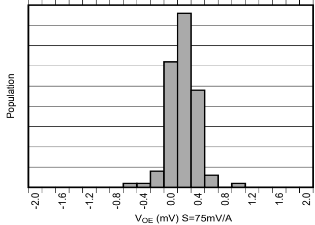
Figure 6-8. Offset Error Production Distribution
