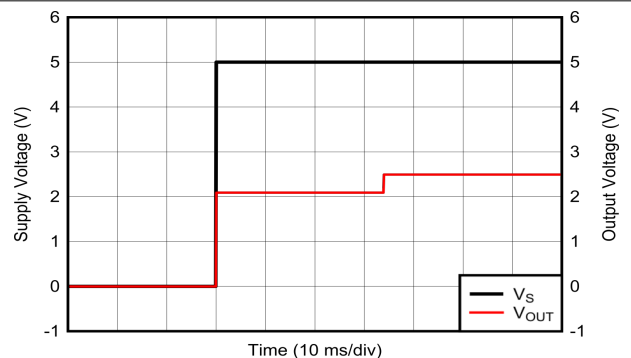
Figure 6-20. Startup Transient Response
