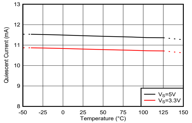
Figure 6-22. Quiescent Current vs Temperature
