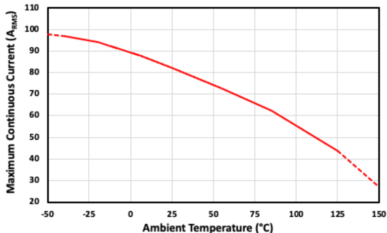
Figure 7-4. Maximum Continuous RMS Current vs Ambient Temperature
