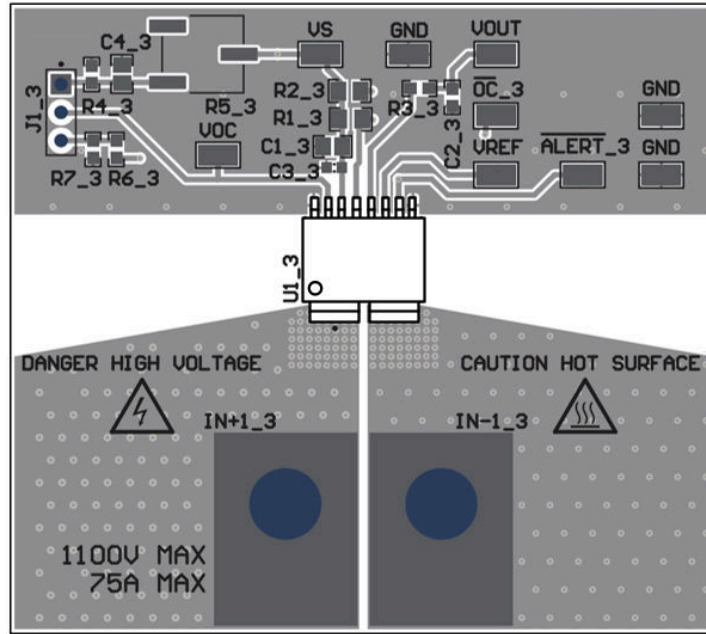
Figure 9-4. Recommended Board Layout
