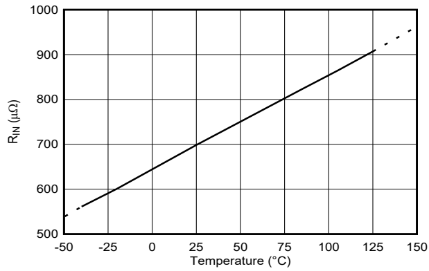
Figure 6-23. Input Conductor Resistance vs Temperature
