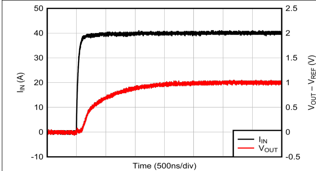
Figure 6-17. Voltage Output Step Response, Rising
