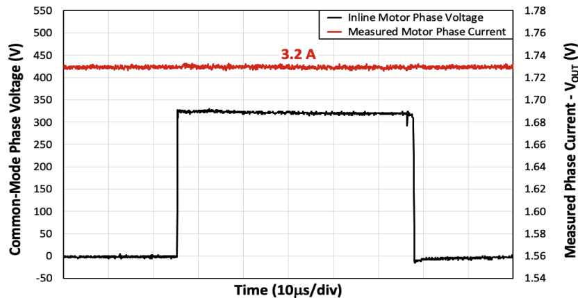
Figure 9-3. Inline Motor Current-Sense Input and Output Signals
