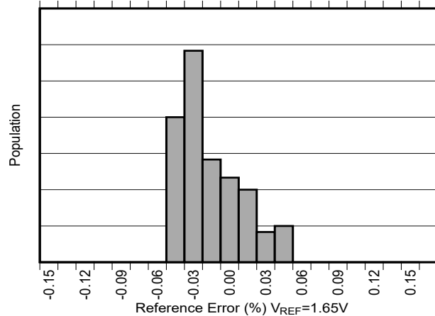
Figure 6-11. Reference Error Production Distribution
