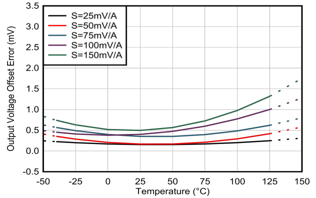
Figure 6-2. Offset Error vs Temperature
