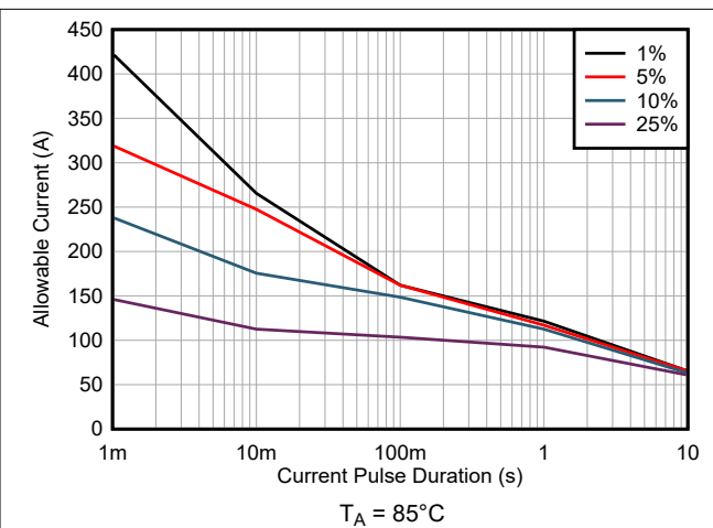
Figure 7-6. Maximum Repetitive Pulsed Current vs. Pulse Duration
