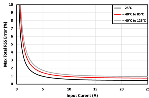
Figure 9-1. RSS Error vs Input Current
