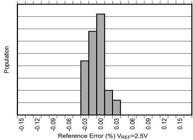
Figure 6-10. Reference Error Production Distribution
