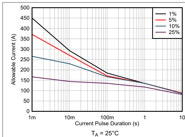
Figure 7-5. Maximum Repetitive Pulsed Current vs. Pulse Duration
