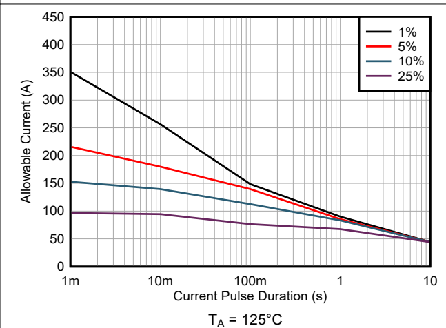
Figure 7-8. Maximum Repetitive Pulsed Current vs. Pulse Duration
