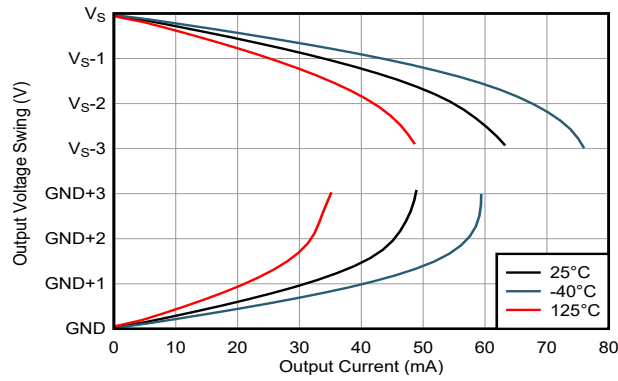
Figure 6-21. Output Swing vs Output Current
