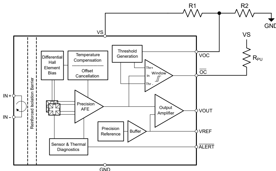
Figure 8-5. User Configurable Overcurrent Threshold
