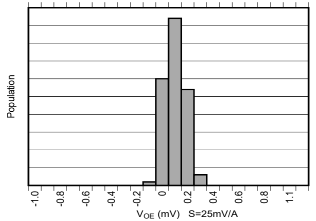
Figure 6-6. Offset Error Production Distribution
