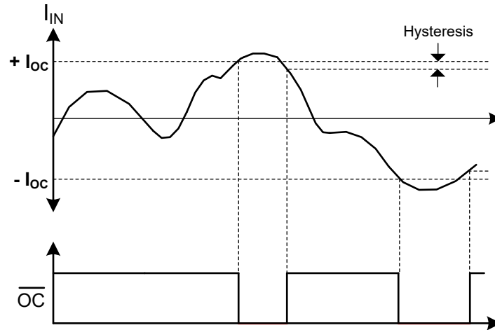
Figure 8-6. Overcurrent Detection Diagram
