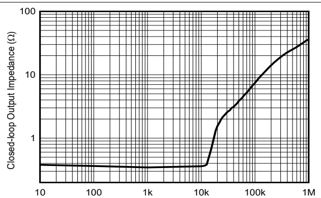
Figure 6-16. Output Impedance vs Frequency
