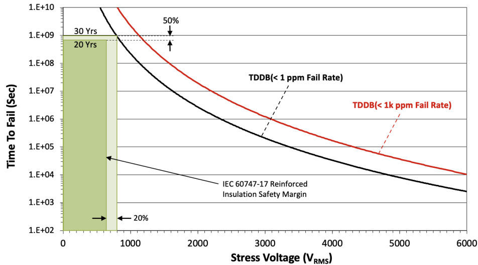
Figure 8-1. Insulation Lifetime
