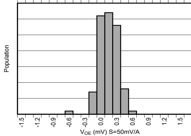
Figure 6-7. Offset Error Production Distribution
