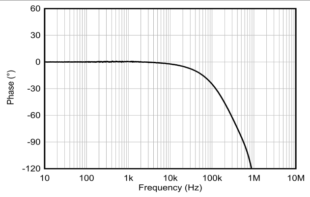
Figure 6-14. Phase vs Frequency, All Gains
