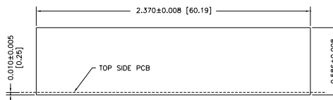
Panel cutout
