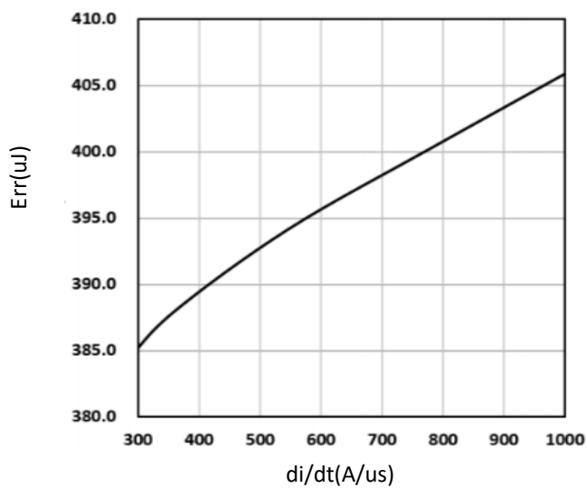
开关损耗二极管 Switching losses Diode Err = f(di/dt) V_{GE}=15V, I_C=15A, V_{CE}=600V
