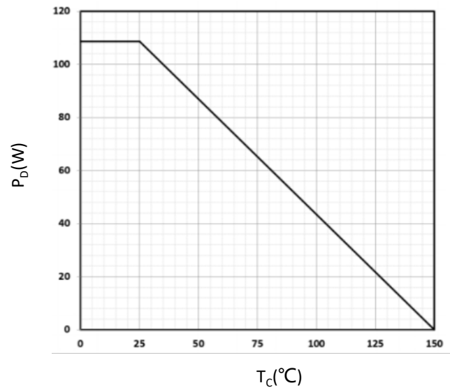
功耗 Power dissipation as a function of case temperature P_D=f(T_c)
