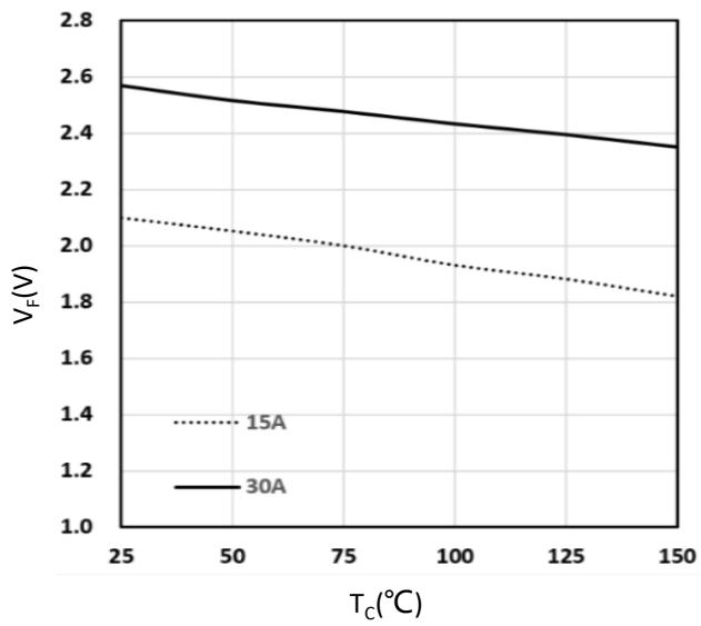
正向偏压二极管 Diode forward voltage as a function of junction temperature
