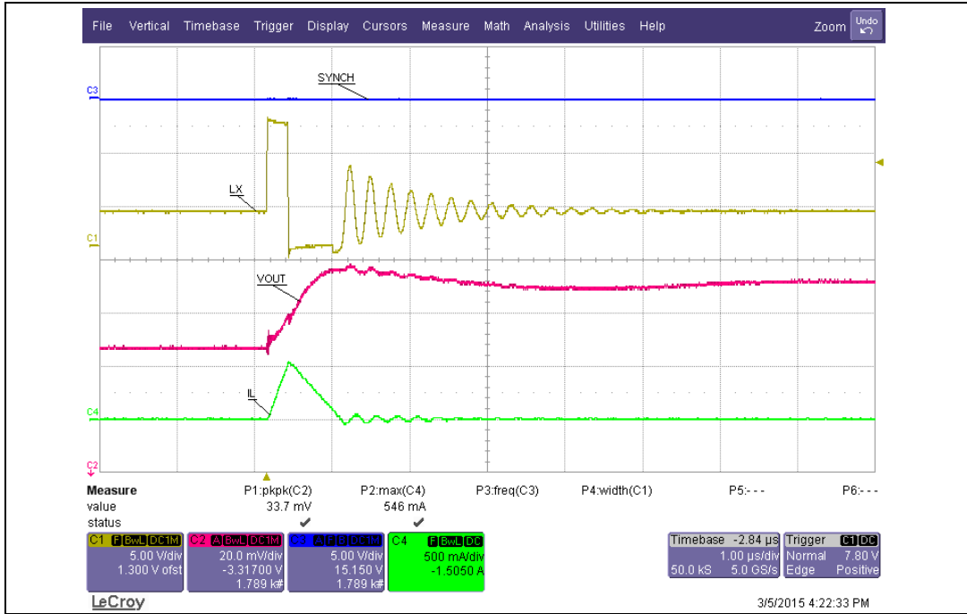
Figure 20. LCM operation with ISKIP_H = 350\text{ mA typ. at zero load}
