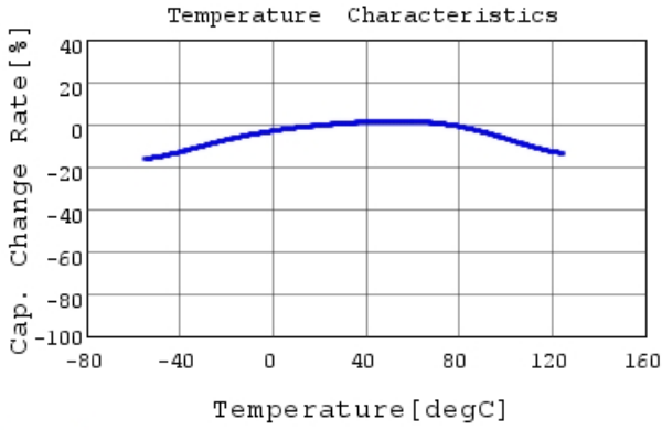
GRT033C71C104KE01 C-Temp. capchange, DC0.0V,
