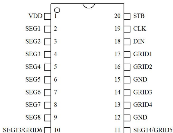
AIP1620 SOP-20
