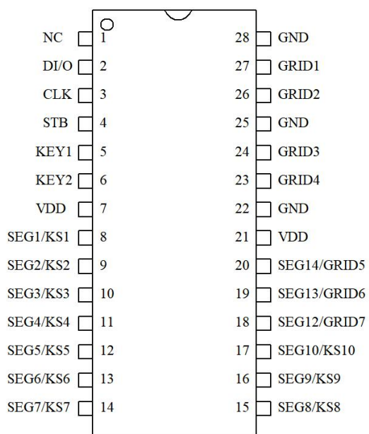
AIP1628 SOP/SSOP-28
