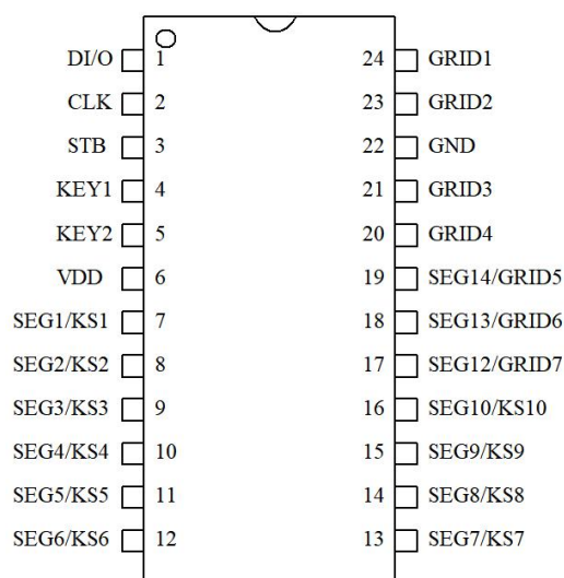
AIP1668 SOP/SSOP-24
