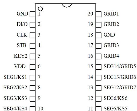
AIP1620B SOP-20
