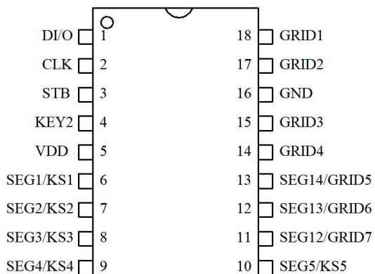
AIP1618 SOP-18
