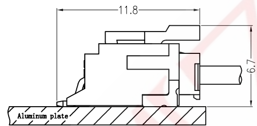
Assembly Layout
