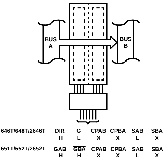
FIGURE 2. REAL-TIME TRANSFER BUS A TO B
