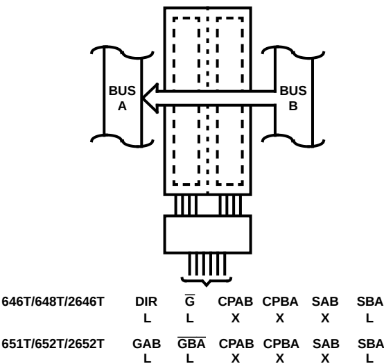
FIGURE 1. REAL-TIME TRANSFER BUS B TO A
