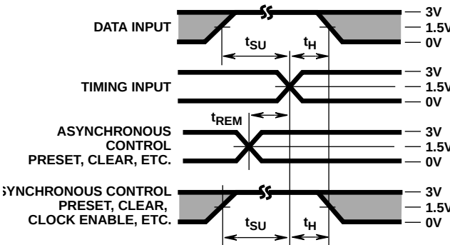
FIGURE 6. SETUP, HOLD, AND RELEASE TIMING
