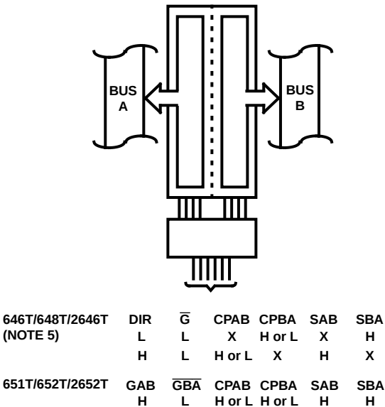
FIGURE 4. TRANSFER STORES DATA TO A AND/OR B
