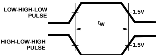
FIGURE 7. PULSE WIDTH
