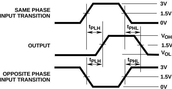
FIGURE 9. PROPAGATION DELAY
