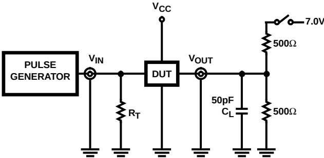
FIGURE 5. TEST CIRCUIT
