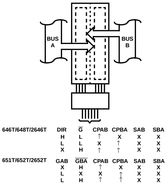
FIGURE 3. STORAGE FROM A AND/OR B
