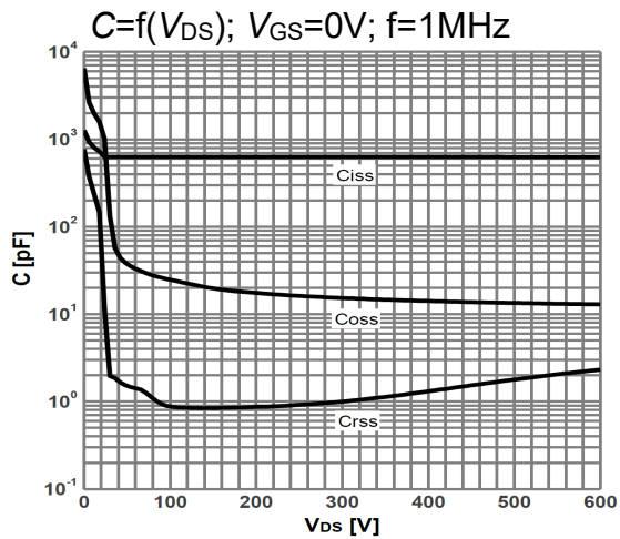
Figure 15: Typ. capacitances
