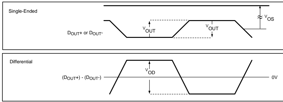
Figure 6. Serializer VOD Diagram
