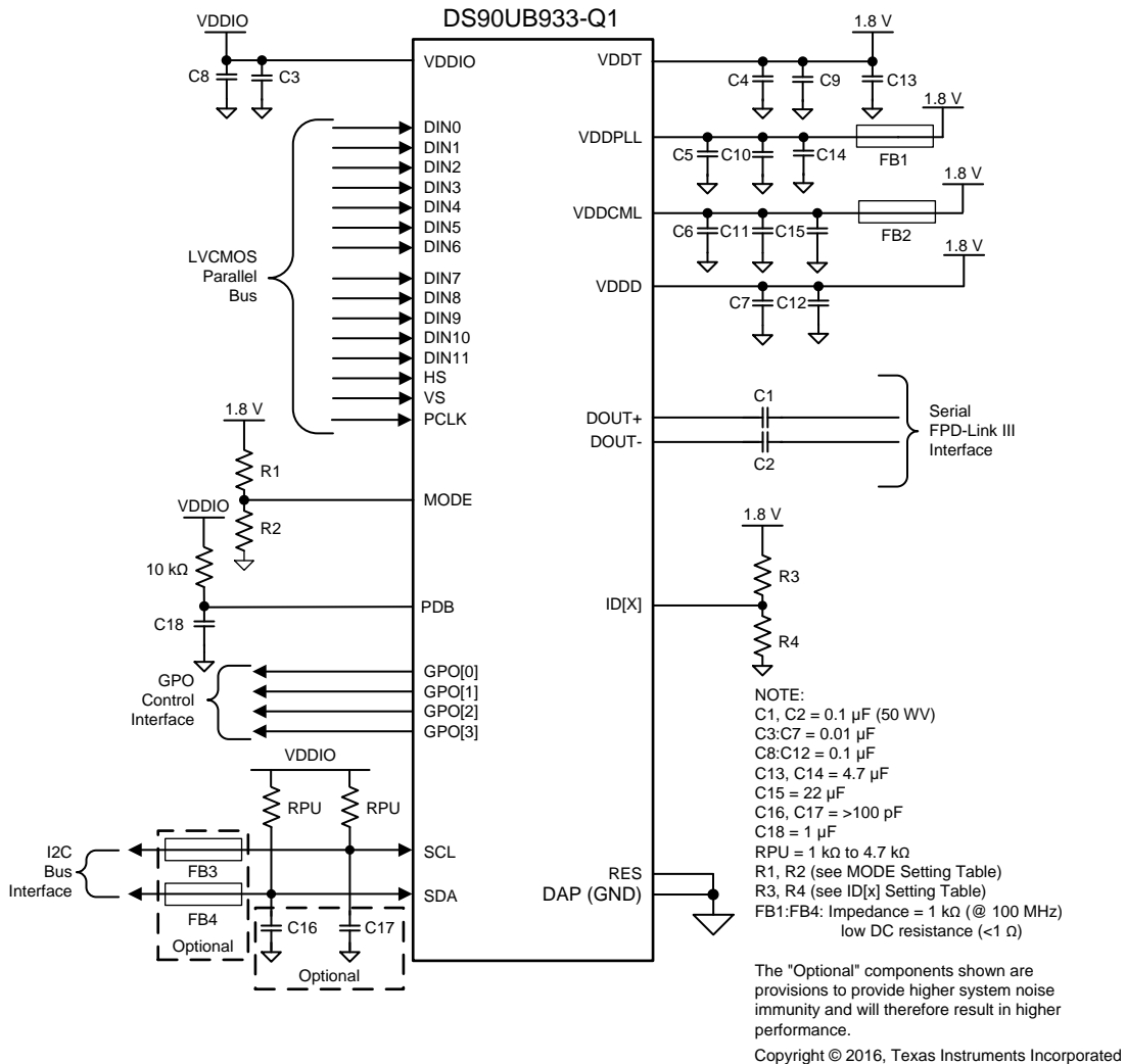
Figure 35. STP Application Connection Diagram
