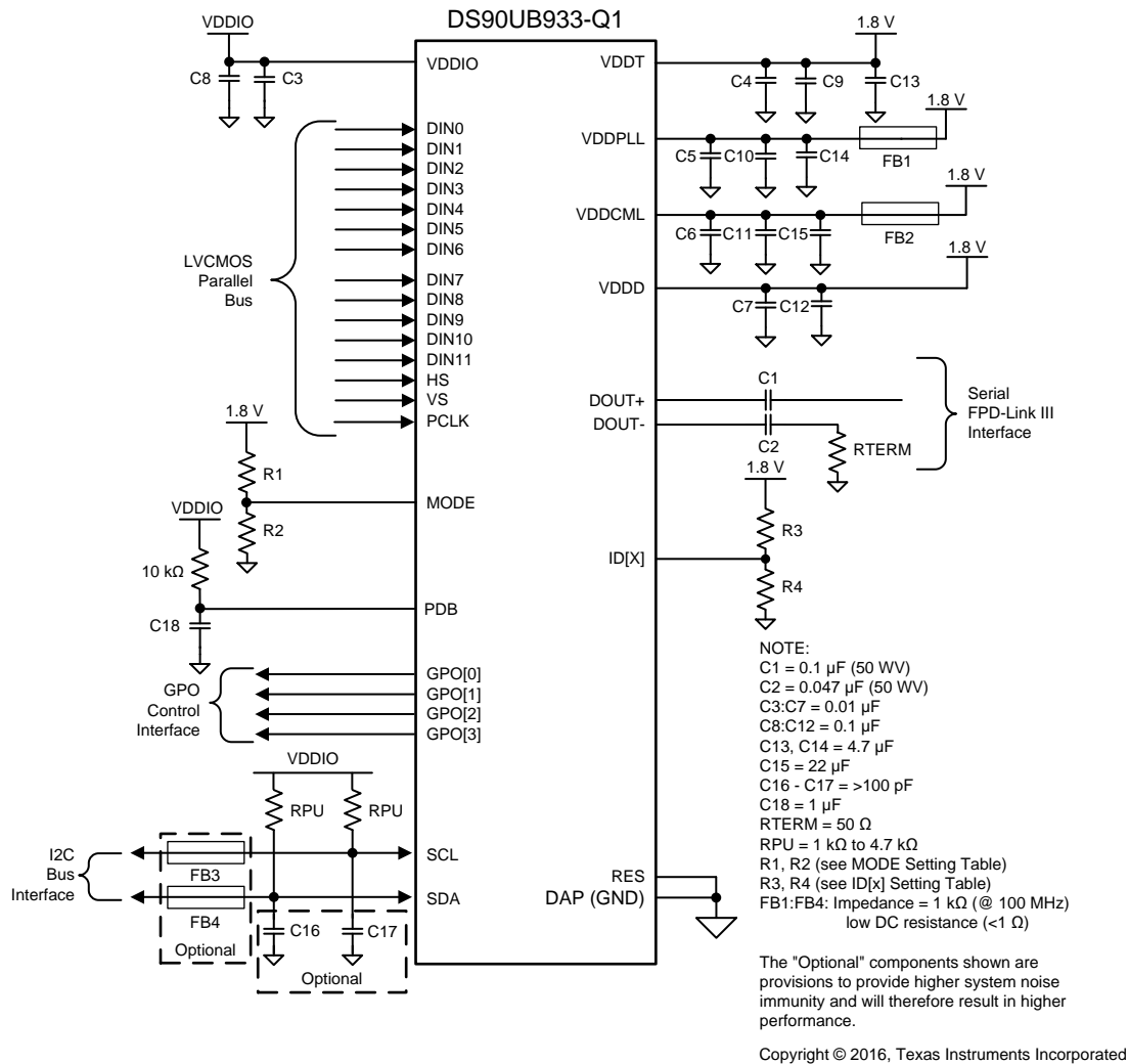
Figure 31. Coax Application Connection Diagram
