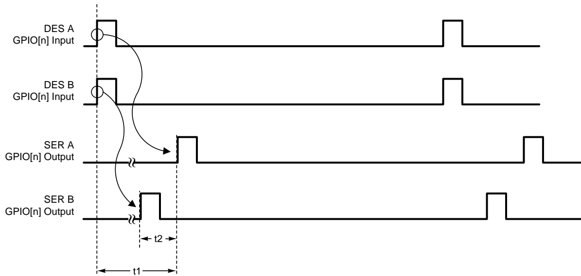
Figure 14. GPIO Delta Latency
