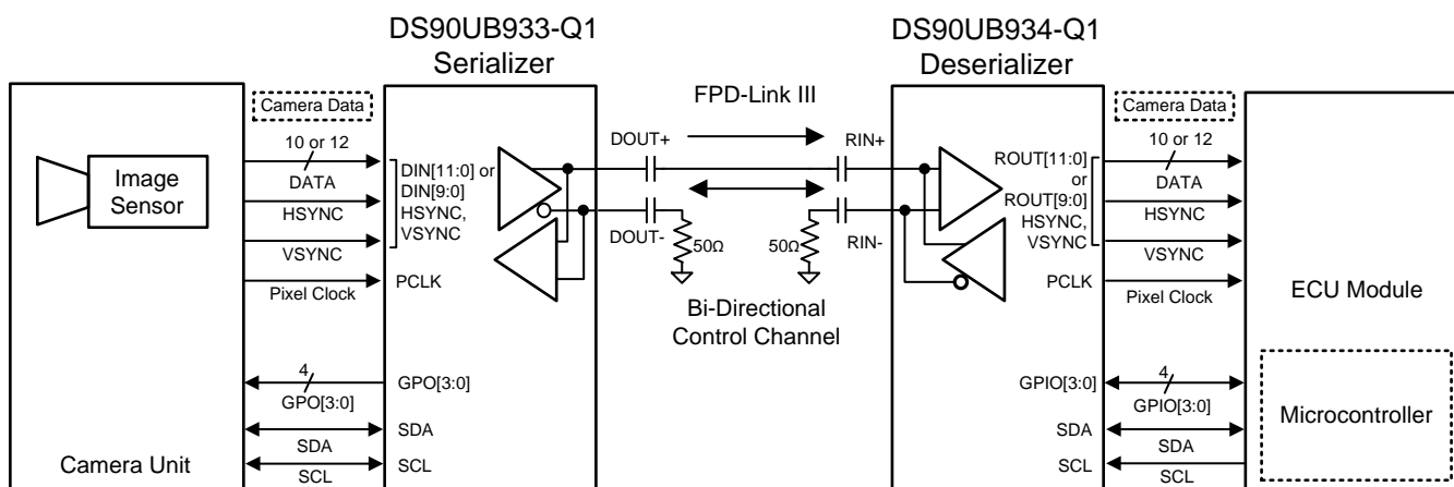
Figure 32. Coax Application Block Diagram
