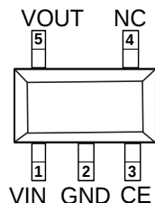
SOT-23-5L(TSOP-5-1.5mm)
