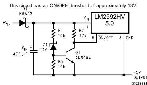
FIGURE 23. Undervoltage Lockout for Inverting Regulator
