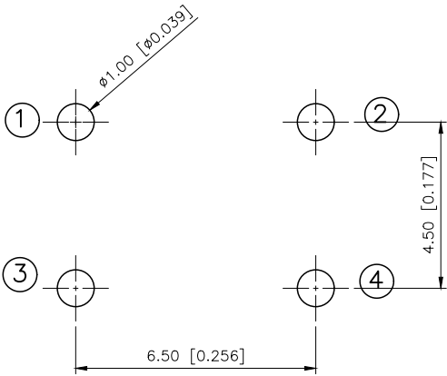
PCB.WELDING DRAWING
