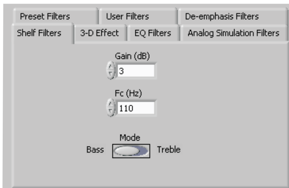
Figure 20. Shelf Filters
