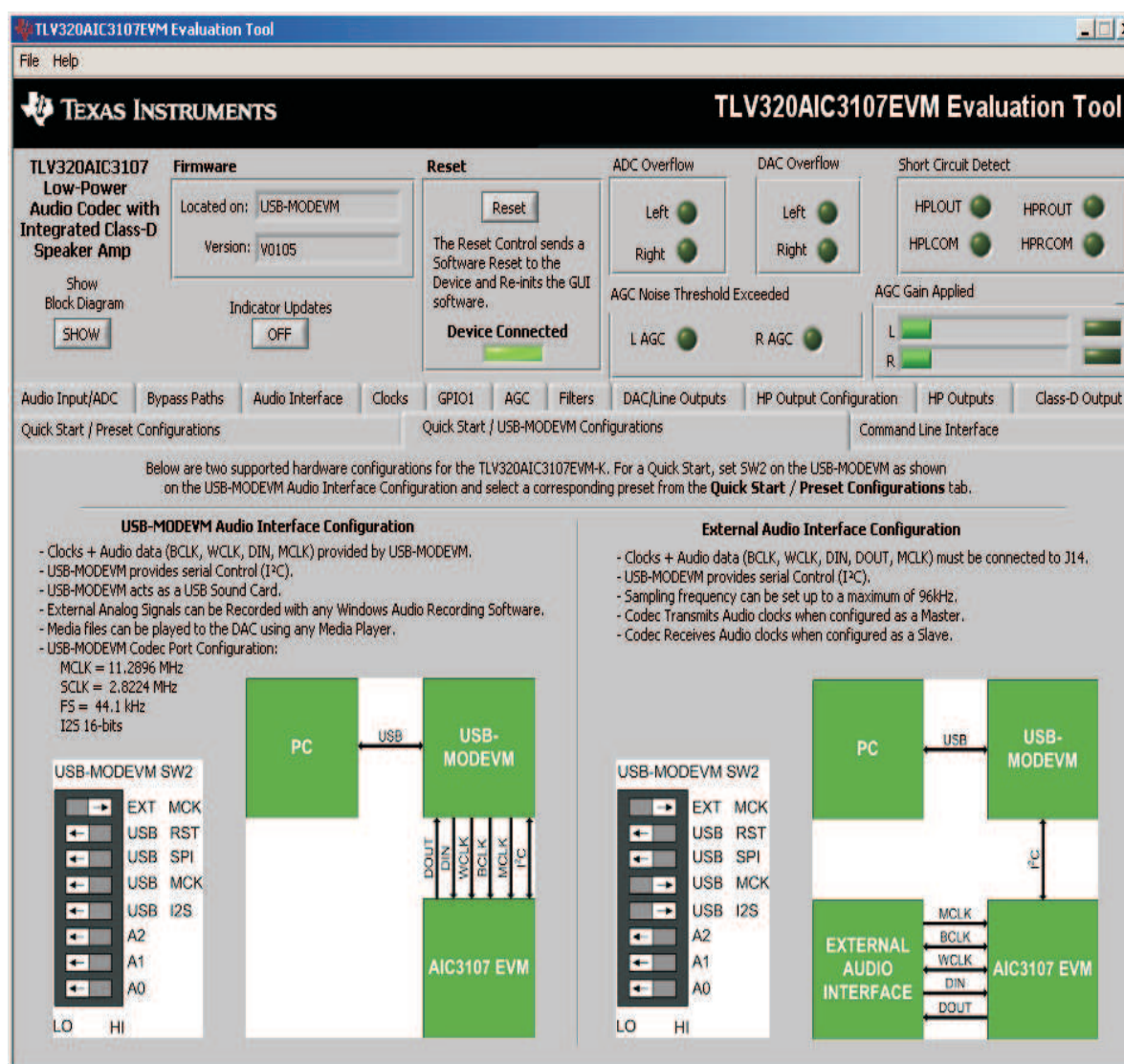
Figure 4. Main Software Screen
