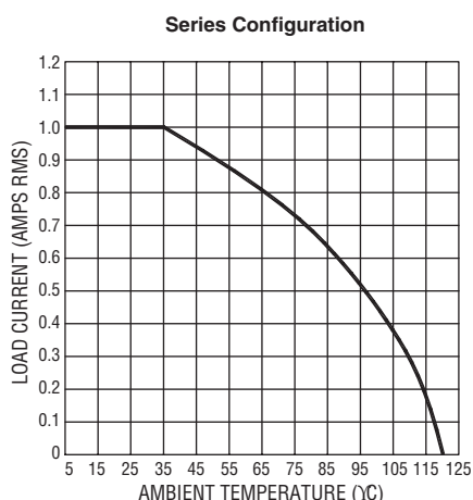
Figure 2 - Temperature Derating Curves
