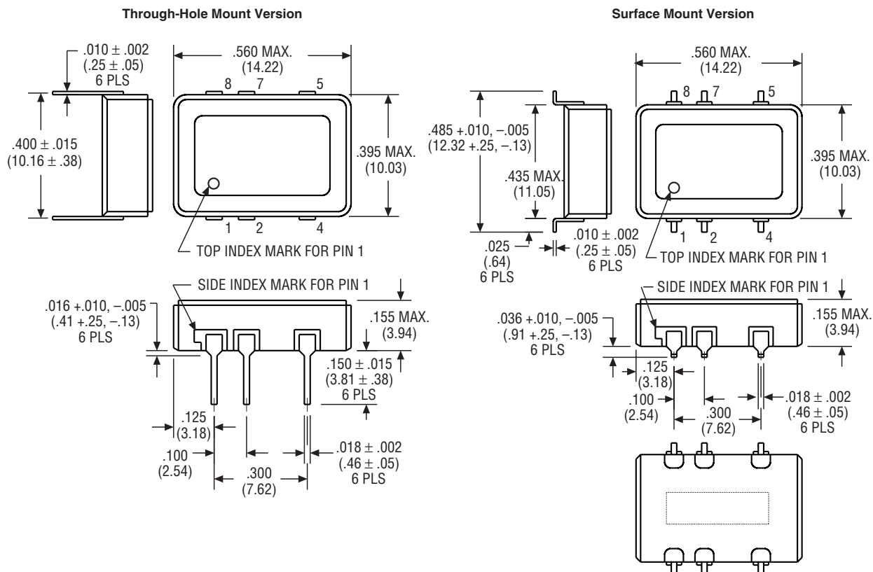
Figure 7 - Outline Dimensions
