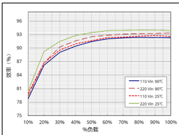
效率 ( V_{out}=50V , T=25^{\circ}C/90^{\circ}C )
