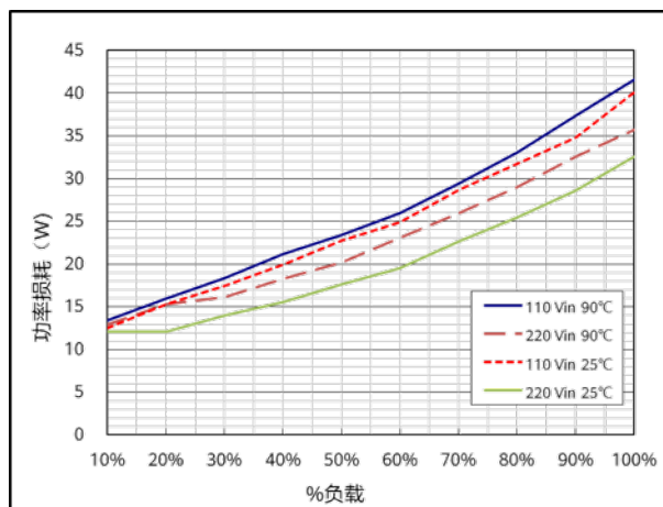
功率损耗 ( V_{out}=50V , T=25^{\circ}C/90^{\circ}C )
