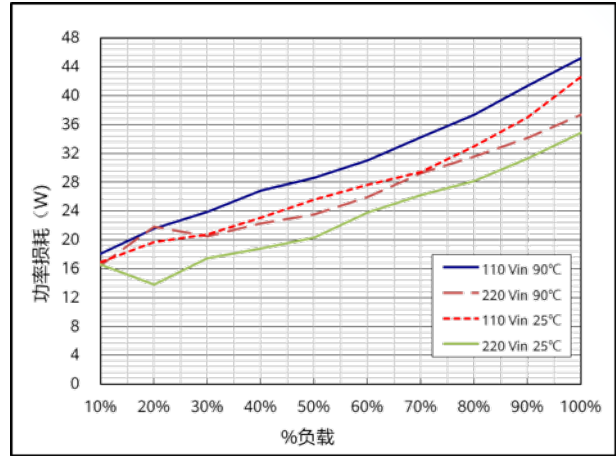
功率损耗 ( V_{out}=55V , T=25^{\circ}C/90^{\circ}C )
