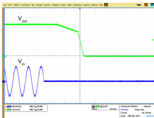
关机 ( V_{in}=220V AC, V_{out}=50V DC)
