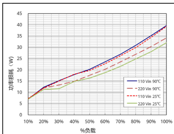
功率损耗 ( V_{out}=42V , T=25^{\circ}C/90^{\circ}C )
