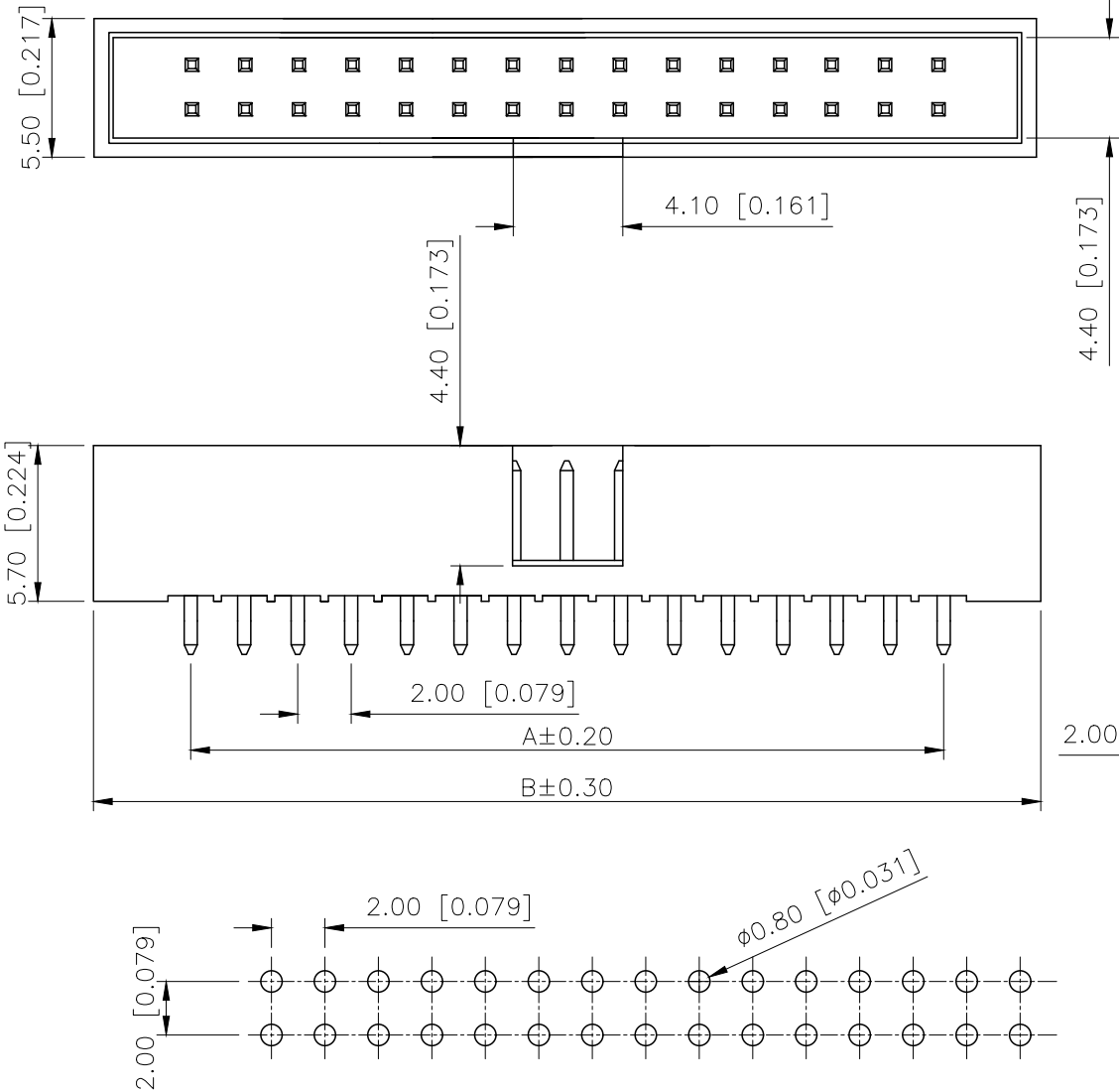
PCB LAYOUT
