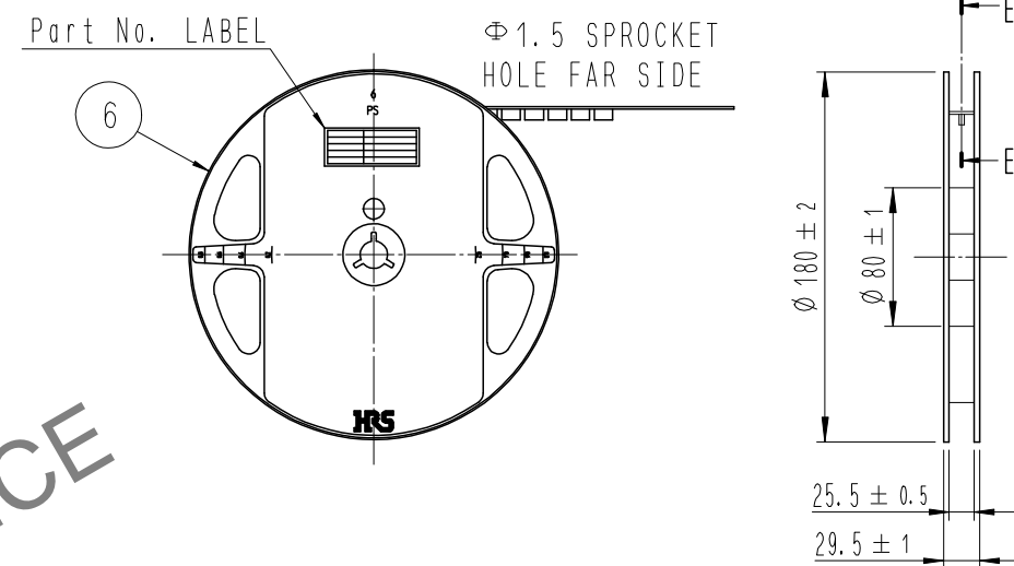
E-E (FREE)
